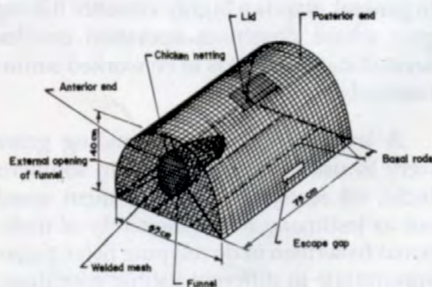
Fig. 3. Modern lobster trap
