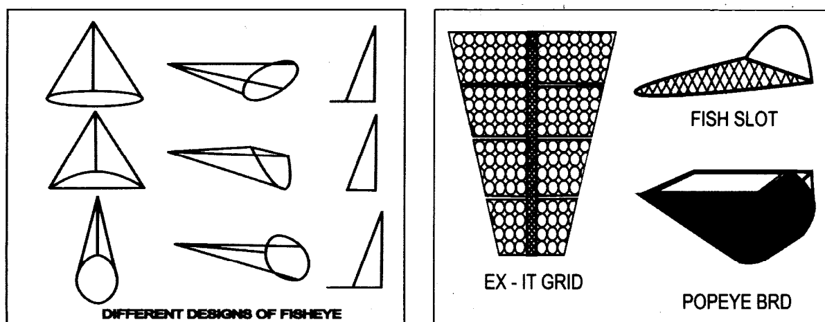
Fig. 8. BRDs with rigid escape opening
